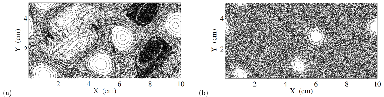
FIG. 12. Mixing by the time-periodic flow P_3 . The distribution of 6 \times 10^4 tracers and the stream lines of the instantaneous flow at t = 317 s (a) and t = 3500 s (b).
