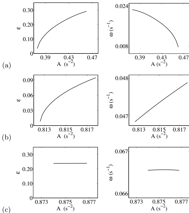
FIG. 4. The perturbation amplitude \epsilon and frequency \omega_1 = 2\pi/T of the time-periodic flows P_1 (a), P_2 (b), and P_3 (c). Only the ranges of A are shown where these flows exist and are stable.
