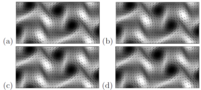
FIG. 6. Time-periodic flow P_2 at A = 0.817 s^{-2} and (a) t=0 , (b) t=T/4 , (c) t=T/2 , (d) t=3T/4 with T = 131.76 s . The same color bar as in Fig. 5(a) is used here.
