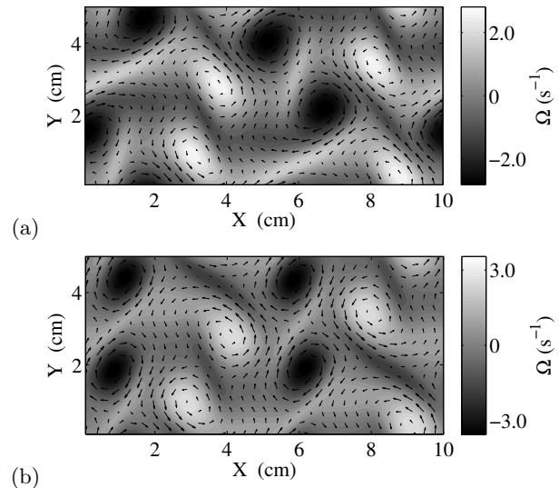
FIG. 5. Stable steady flow N (a) and unstable steady flow S (b) at A = 0.750 s^{-2} .
