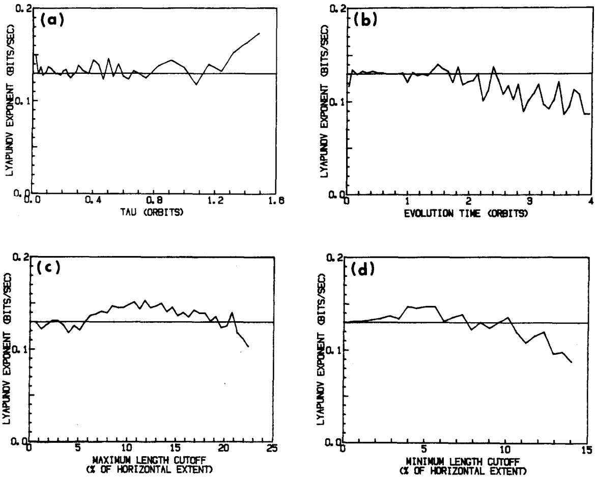
Fig. 6. Stationarity of \lambda_1 for Rossler attractor data (8192 points spanning 135 orbits) for the fixed evolution time program is shown for the input parameters: a) Tau (delay time); b) evolution time between replacement steps; c) maximum length of replacement vector length allowed; and d) minimum length of replacement vector allowed. The correct value of the positive exponent is 0.13 bits/s and is shown by the horizontal line in these figures.
